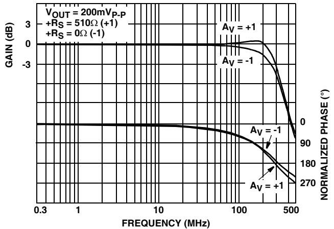
FIGURE 12. FREQUENCY RESPONSE
