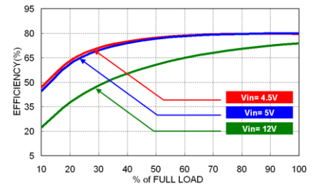
MPS(H)02-05S05 Efficiency vs. Output Current
