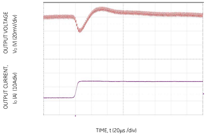
Figure 22. Transient Response to Dynamic Load Change from 50% to 100% at 12Vin, C_{out} = 2 \times 47 \mu F + 1 \times 330 \mu F , C_{Tune} = 3300 pF & R_{Tune} = 240 \Omega
