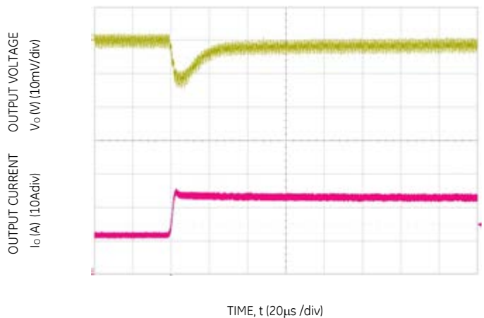
Figure 10. Transient Response to Dynamic Load Change from 50% to 100% at 12Vin, Cout= TBD, CTune=TBD & RTune=TBD
