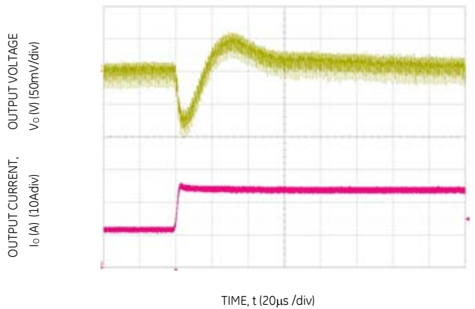
Figure 28. Transient Response to Dynamic Load Change from 50% to 100% at 12V in , C out = 2x47uF+1x330uF, CTune=2700pF & RTune=300Ω
