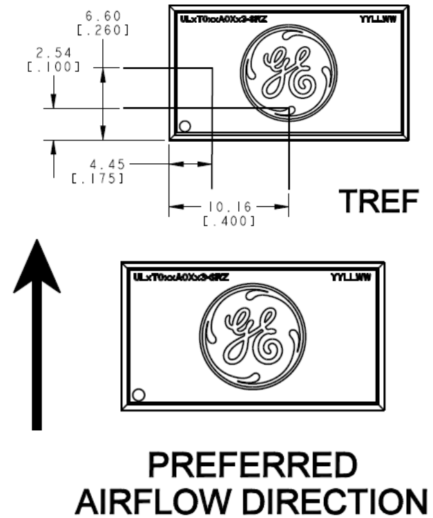
Figure 48. Preferred airflow direction and location of hot-spot of the module ( T_{ref} ).
