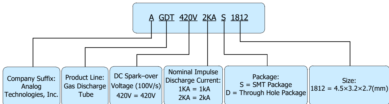
Naming Principle of AGDT420V2KAS1812
