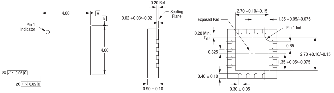
Figure 13. SKY13286-359LF 16-Pin QFN Package Dimensions
