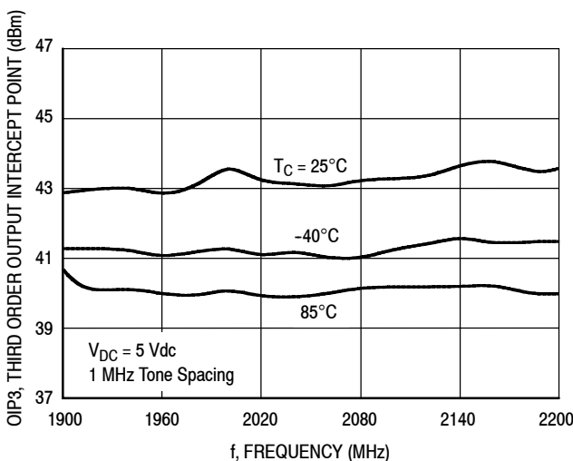
Figure 21. Third Order Output Intercept Point versus Frequency
