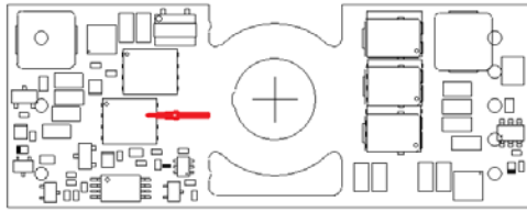
Figure 15. Temperature Monitoring Locations
