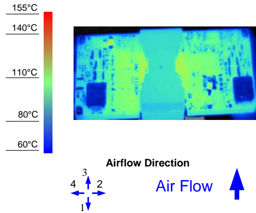
Figure 8. Thermal Image for Airflow Direction 3 (4A output, 55°C ambient, 200 LFM, typical Vin, open frame)
